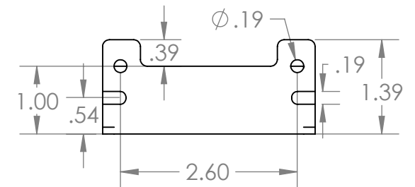
VIEW A: MOUNTING FOOT DETAIL
