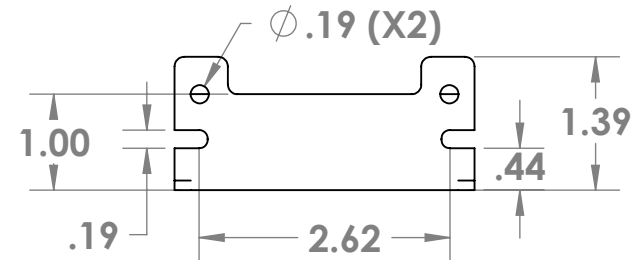
VIEW A: MOUNTING FOOT DETAIL
